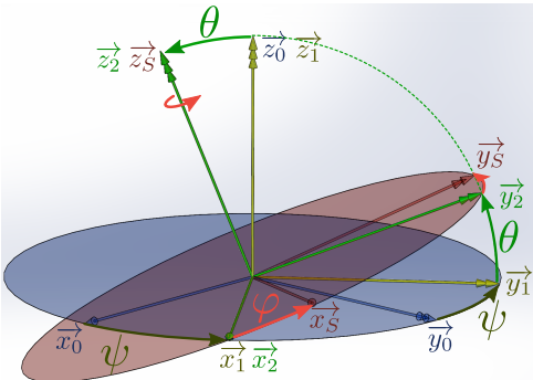
(c) Angle de rotation propre \varphi = (\vec{y}_2, \vec{y}_S) = (\vec{x}_2, \vec{x}_S)
