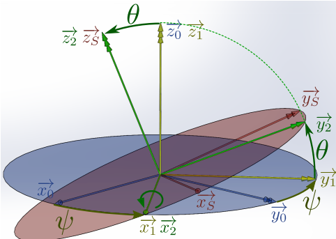
(b) Angle de nutation \theta = (\vec{y}_1, \vec{y}_2) = (\vec{z}_1, \vec{z}_2 = \vec{z}_S)
